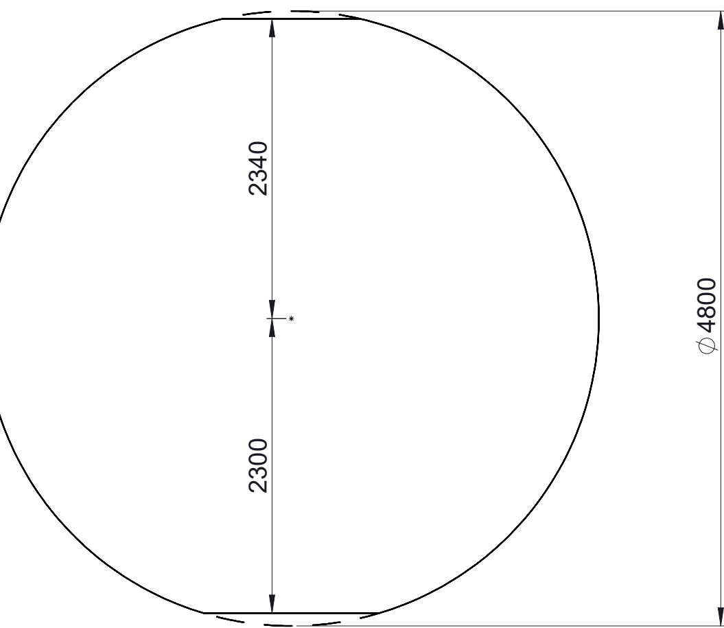
APC B SAGOMATURA PEZZO / WORKPIECE SHAPE
