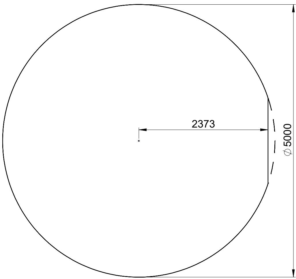
APC D SAGOMATURA PEZZO / WORKPIECE SHAPE
