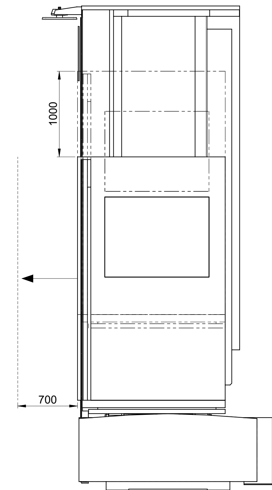
CORSE PEDANA OPERATORE OPERATOR PLATFORM'S STROKES
