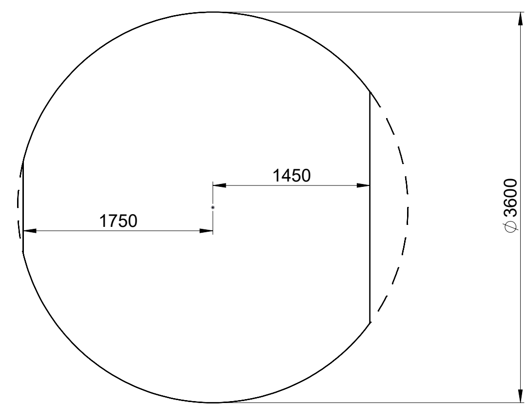
APC D SAGOMATURA PEZZO / WORKPIECE SHAPE
