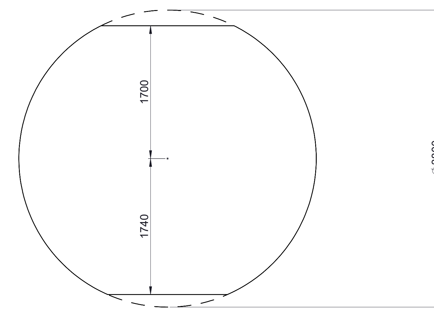
APC A SAGOMATURA PEZZO / WORKPIECE SHAPE
