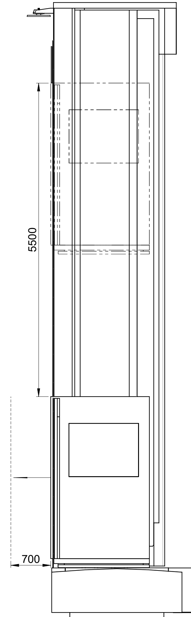
CORSE PEDANA OPERATORE OPERATOR PLATFORM'S STROKES
