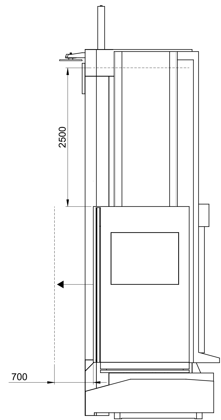
CORSE PEDANA OPERATORE OPERATOR PLATFORM'S STROKES
