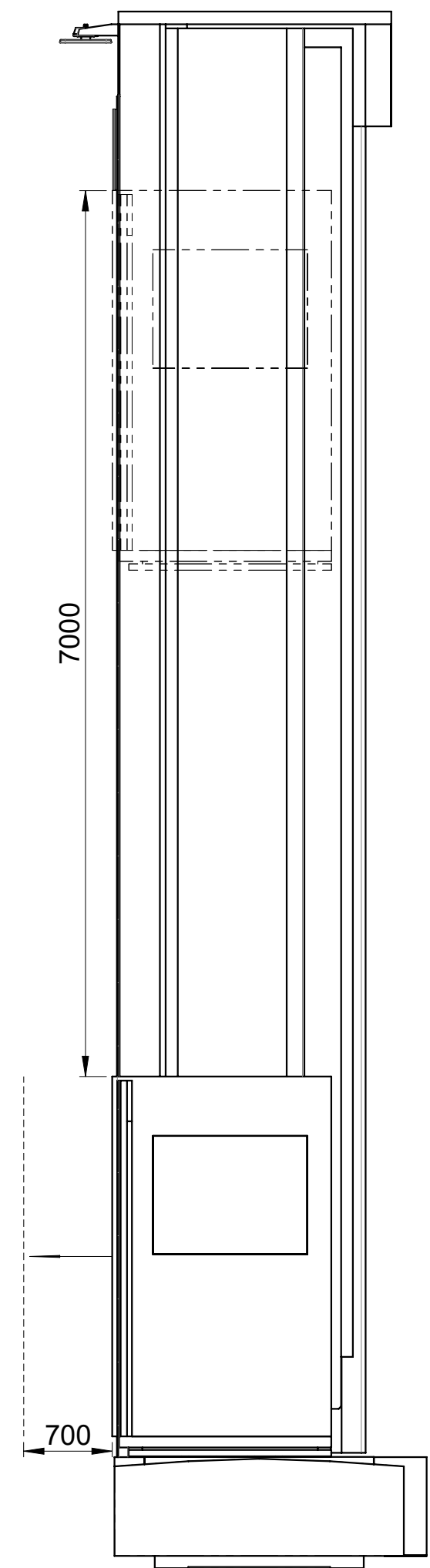
CORSE PEDANA OPERATORE OPERATOR PLATFORM'S STROKES
