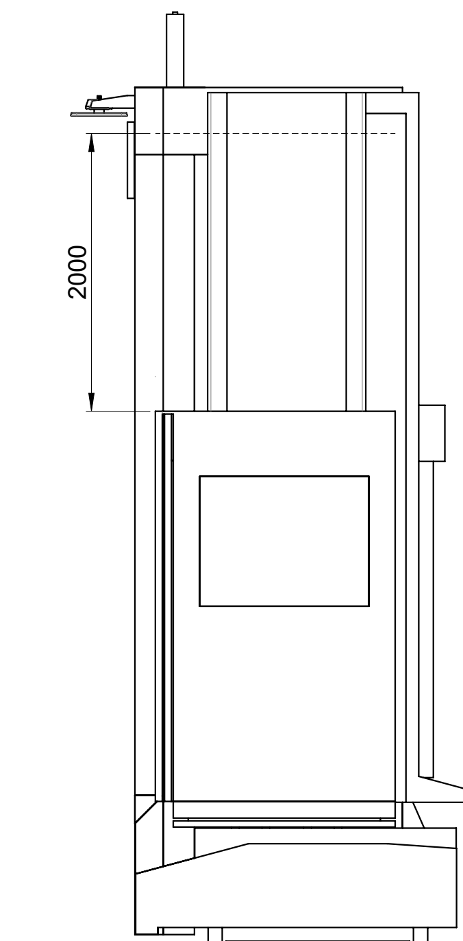
CORSE PEDANA OPERATORE OPERATOR PLATFORM'S STROKES
